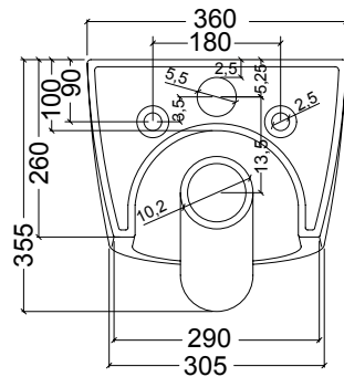
Art. 0652 Vaso Wayd sospeso Wayd wall hung wc bowl
