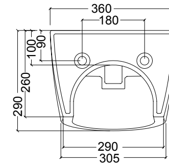
Art. 0752 Bidet sospeso Wayd Wayd wall hung bidet bowl
