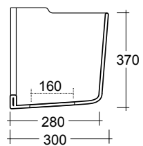
Art. 0950 Semicolonna Soho Soho semi-pedestal
